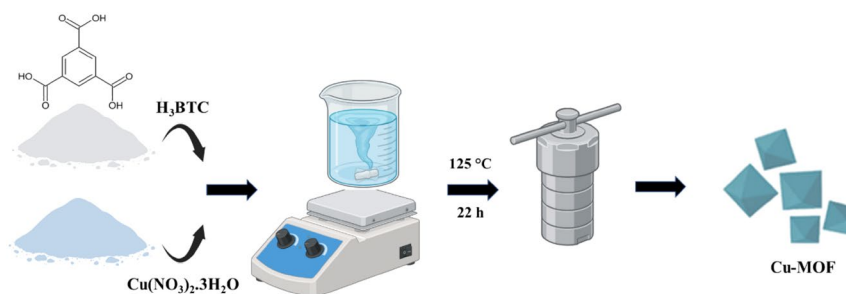
Fig. 3. A schematic illustration of the Cu-MOF fabrication step.
