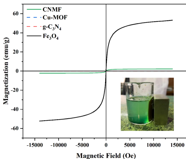
Fig. 8. VSM hysteresis loop at room temperature of \text{Fe}_3\text{O}_4 , \text{g-C}_3\text{N}_4 , Cu-MOF, and CNMF nanocomposites.
