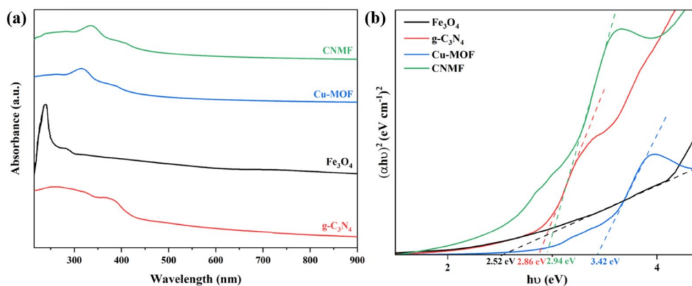
Fig. 7. a) UV-Vis absorption spectra and b) Tauc plots of the as-prepared samples.
