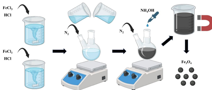
Fig. 2. Schematic of the Fe 3 O 4 NPs synthesis process.
