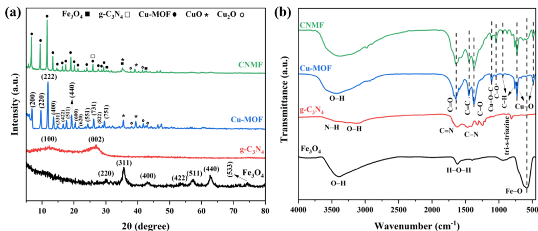
Fig. 5. a) XRD patterns of the synthesized powders and b) FTIR spectra of the as-prepared samples.
