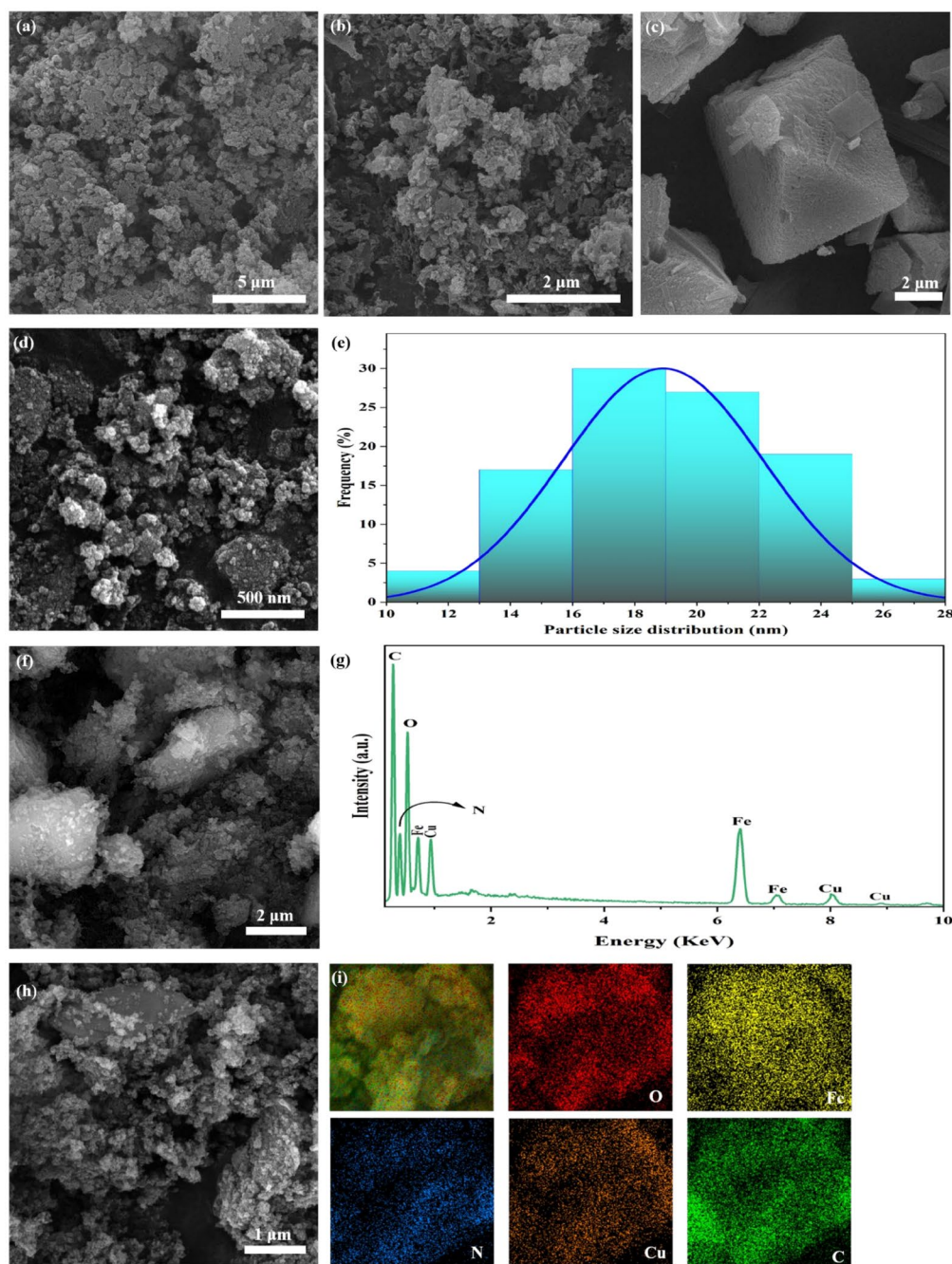
Fig. 6. FE-SEM images of a, b) g-C 3 N 4 , c) Cu-MOF, d) Fe 3 O 4 , and f,h) CNMF composite; e) particle size distribution of Fe 3 O 4 ; g) the EDS spectra of the CNMF composite; and i) elemental mappings of the CNMF composite.
