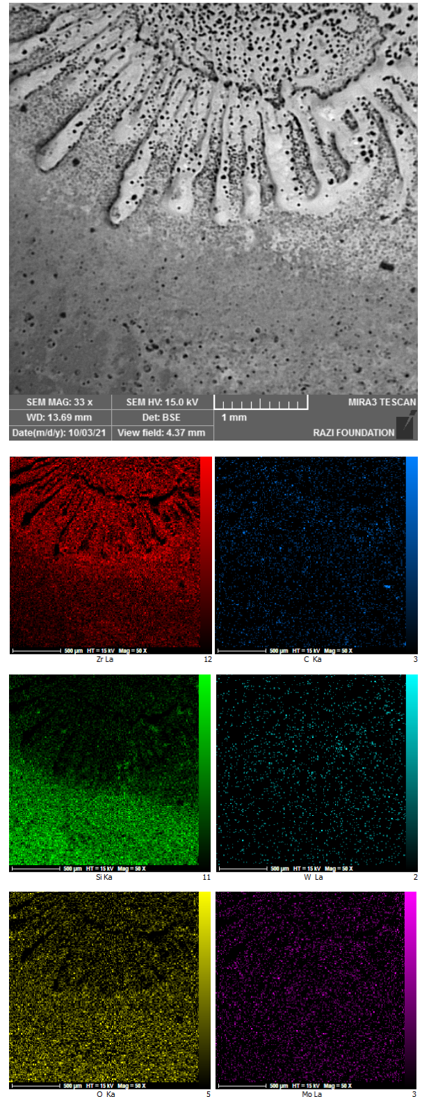
Fig. 12. SEM/EDS data taken from the center and the interface between the middle and central parts of ZSS-3.75WM specimen after 210 s ablation.
